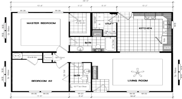
Redwood II 27x38 INS 382F 2 Bedroom, 2 Bath - 1,026 SQ. FT.
